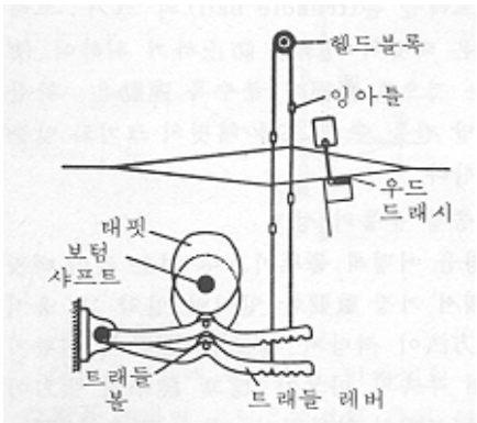
< 4> Heald block
