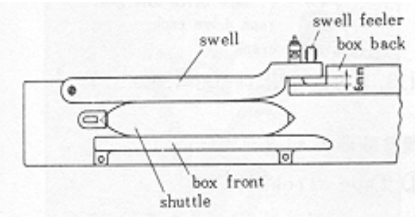
< 11> Shuttle box
