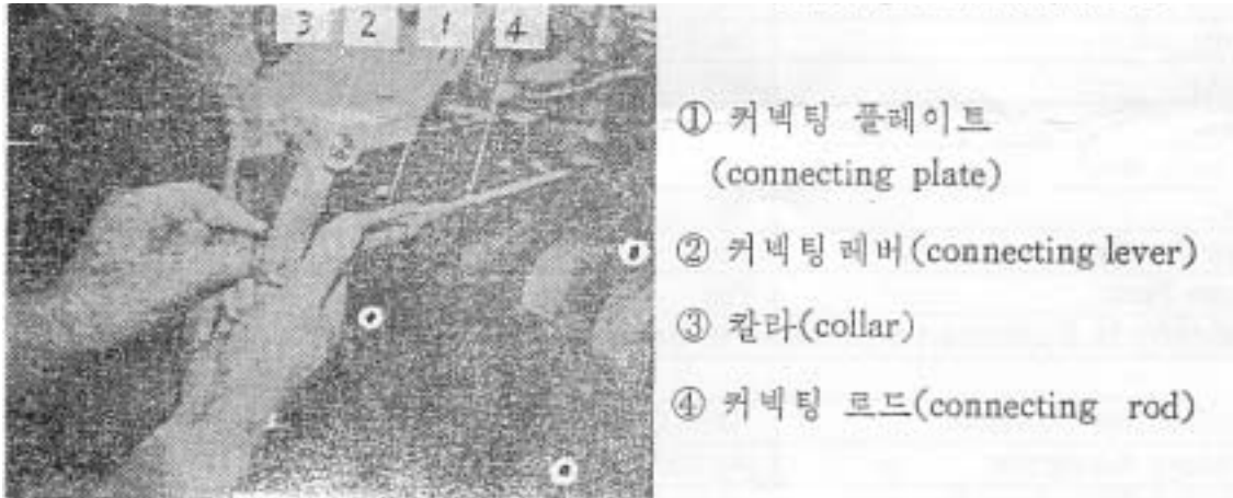
< 5-54> (connecting plate)
