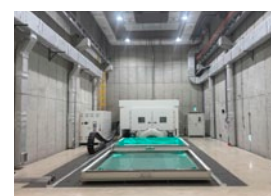
40-ton Combined Vibration Tester
