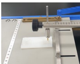
Mercury Lamp Discoloration / Sapphire Scratch Test
