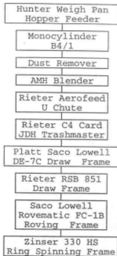
Figure 1: Processing Flow
