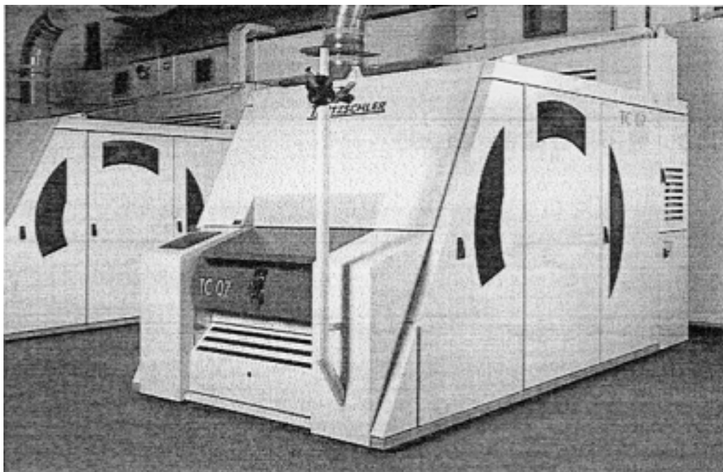
< 4> Trutzschler TC07
