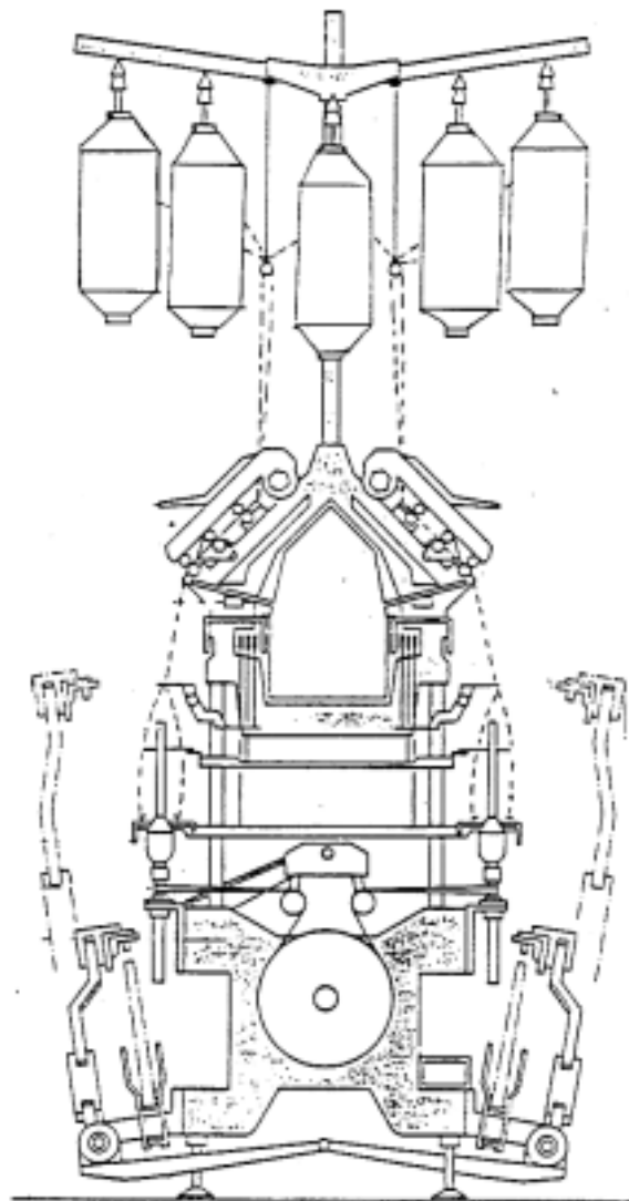
< 78> Rieter G5/1
