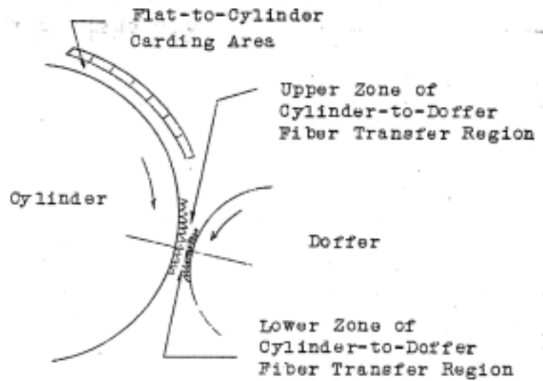
Fig 1. Schematic diagram of cylinder-to-doffer fiber transfer area and flat-to-cylinder carding area.
