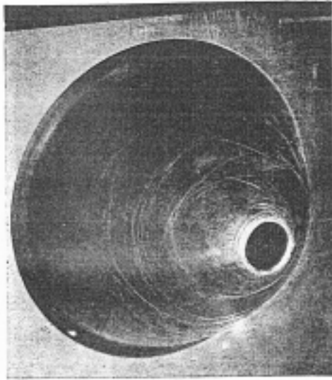
Fig. 6 Spark photograph of everted godet-spinning
