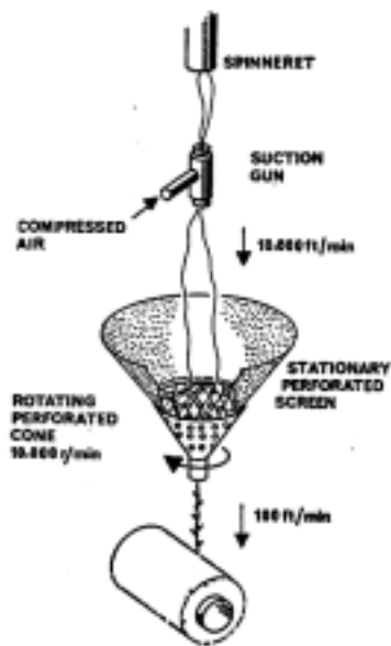
Fig. 1 Cone-spinning
