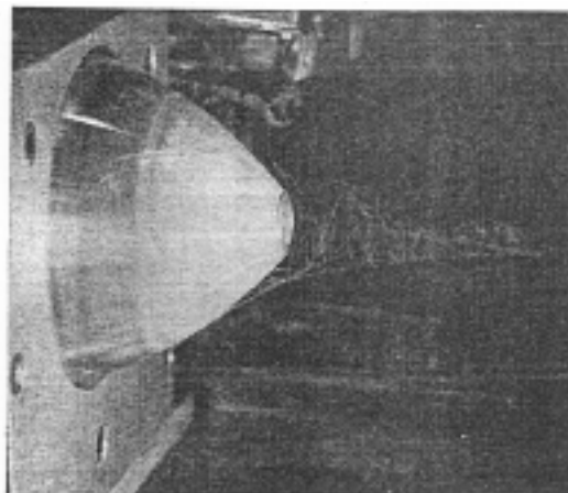
Fig. 4 Spark photograph of godet-spinning
