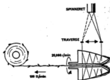
Fig. 5 Everted godet-spinning
