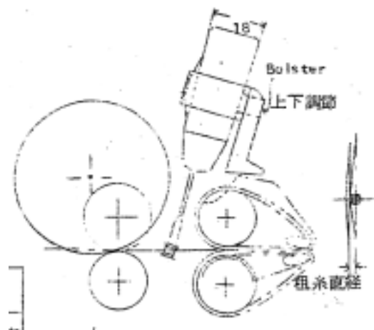
< 2> Draft Tension
