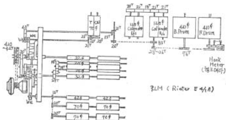
< 1-6> RLM Gearing Diagram (Rieter E4/1A)
