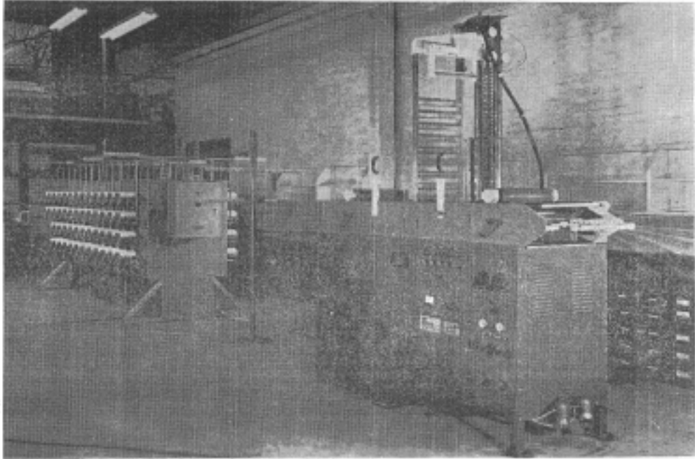
< 1> The Shirley fluid Bed Hot-Stretching Machine and take-up winder. The machine is undergoing trials at Shirley
