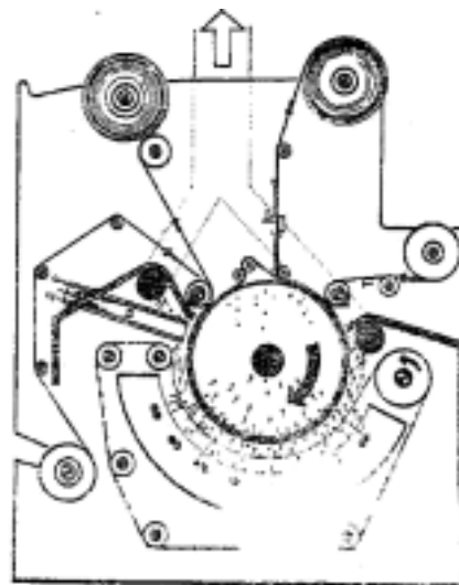
Schematic shows transfer-grinding
