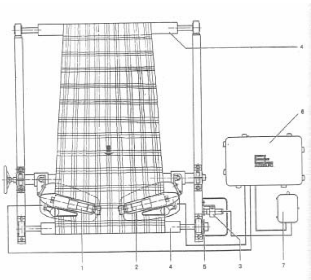
< 2-5> Cloth guiding system
