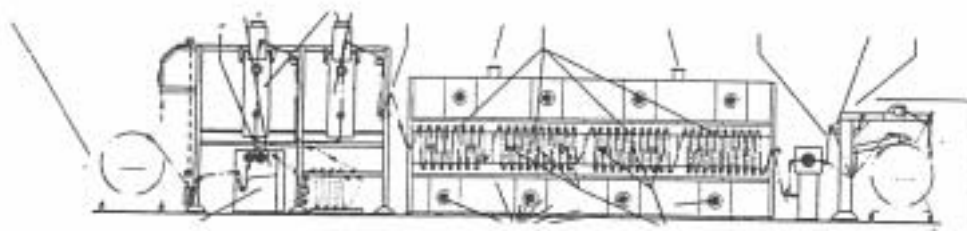
< 2> Pad-Dry, Pad-Dry/thermosol (Monforts)
