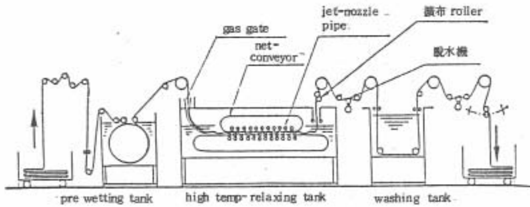
< 7> relaxation machine
