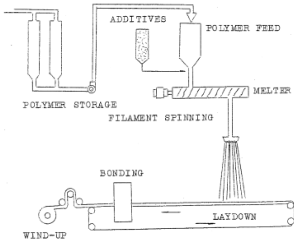
< 2> Schematic of Spunbonded
