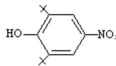
2,6-di-tert-butyl-4-nitrophenol(DBNP)
