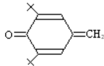
2,6-di-tert-butyl-quinone methide(DBQM)
